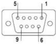
[ GPS device connection(Male) ]
